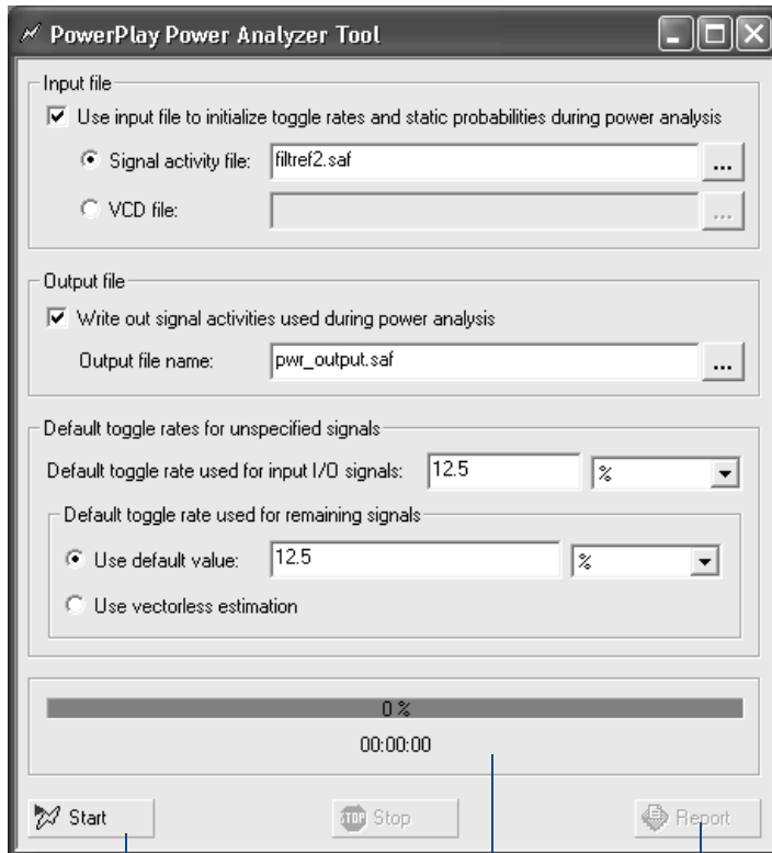
图 2. PowerPlay Power Analyzer Tool
