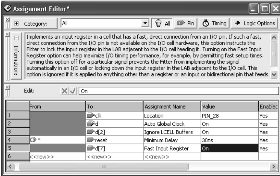
图 2. Quartus II Assignment Editor
