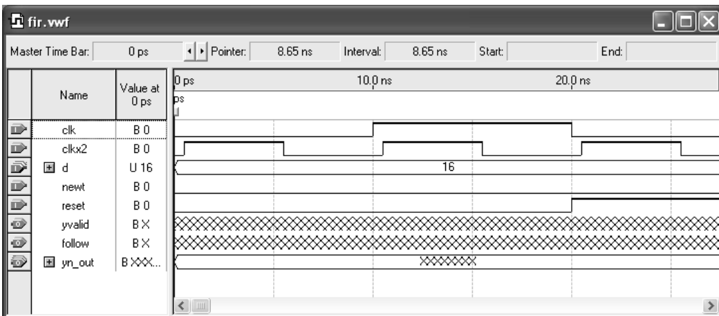
图 4. Quartus II Waveform Editor
