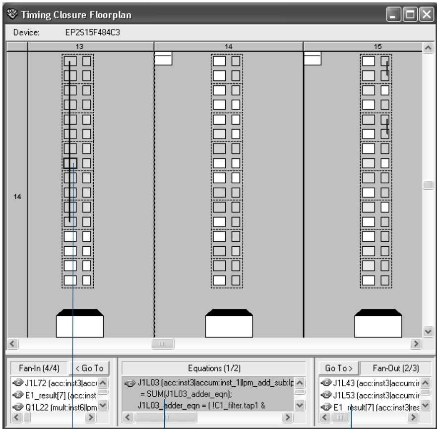
图 5. Timing Closure Floorplan
