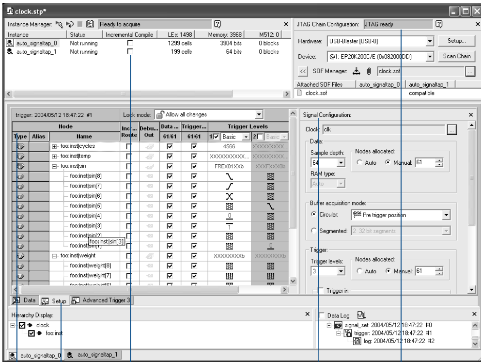
图 3. SignalTap II Logic Analyzer
